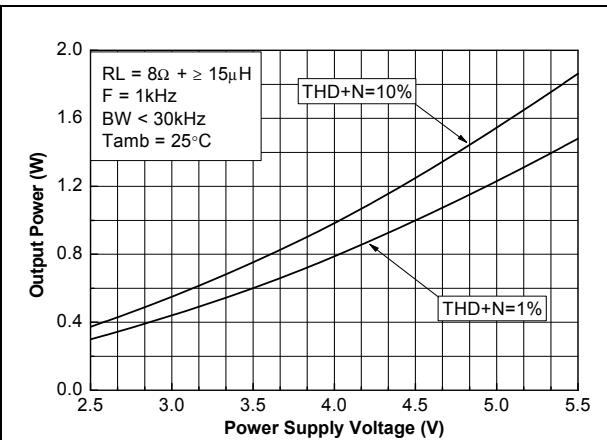
Figure 11. Output power vs. power supply voltage (ii)
